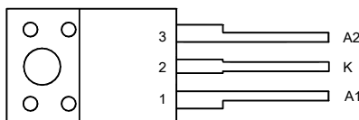
TO-220F-3
