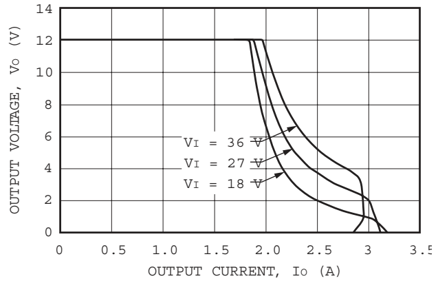
Figure 7. LC020B Typical Output Characteristics, T_A = 25\text{ }^\circ\text{C}
