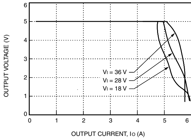
Figure 6. LC020A Typical Output Characteristics, T_A = 25\text{ }^\circ\text{C}
