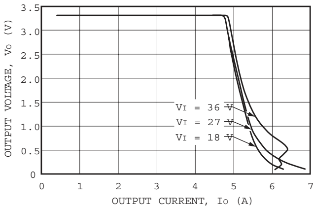
Figure 5. LC020F Typical Output Characteristics, T_A = 25\text{ }^\circ\text{C}
