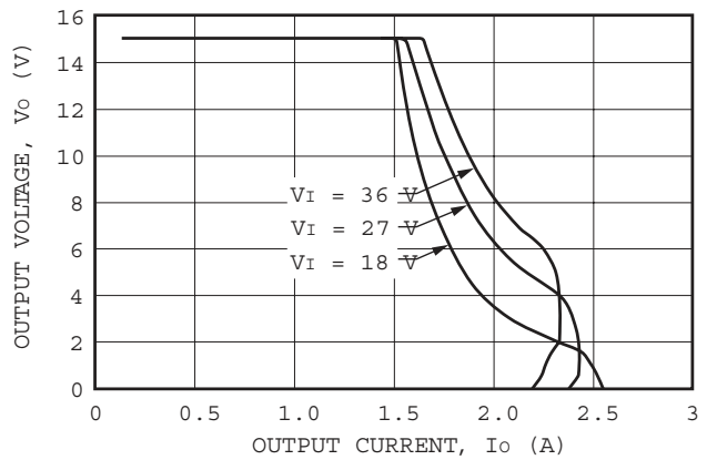
Figure 8. LC020C Typical Output Characteristics, T_A = 25\text{ }^\circ\text{C}
