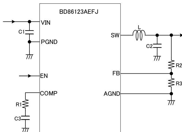
Figure 1. Application Circuit
