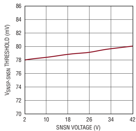
V_{\text{SNSP-SNSN}} Current Limit Threshold vs SNSN Voltage, \text{SNSN} > 2\text{V}
