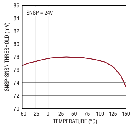
SNSP-SNSN Current Limit Threshold vs Temperature
