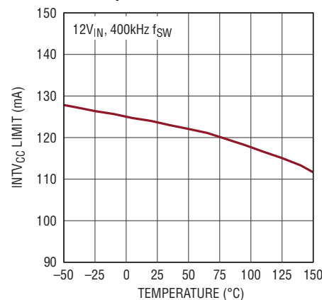
INTV CC Maximum Source Current vs Temperature
