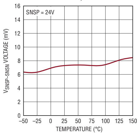
SNSP-SNSN Zero Cross Threshold vs Temperature
