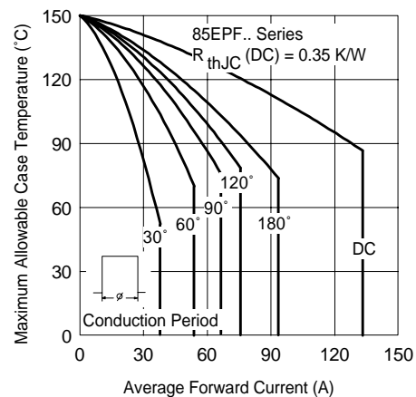
Fig. 2-Current Rating Characteristics
