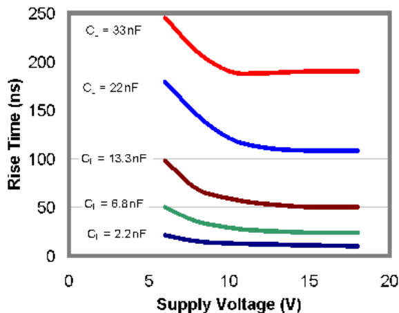
Figure 19. Rise Time vs. Supply Voltage
