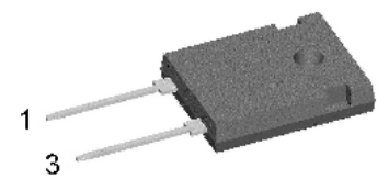
Backside: cathode
