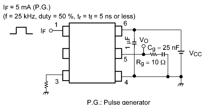
Fig. 13.1.7 Switching Time Test Circuit and Waveform
