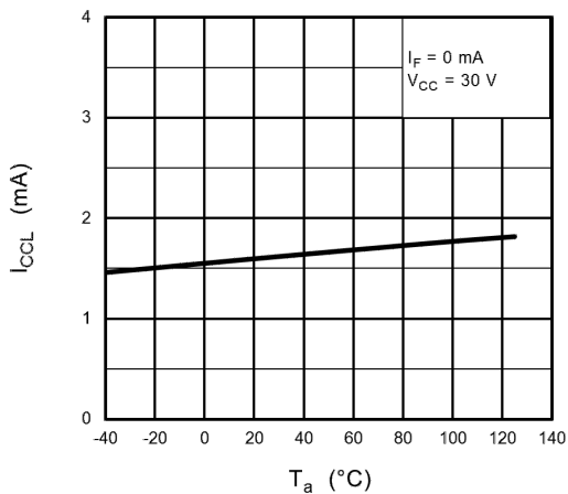
Fig. 13.2.5 I_{cCL} - T_a
