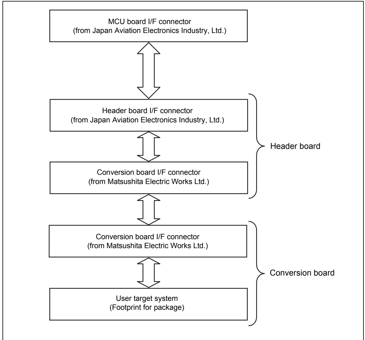
Figure 6-1. Function block diagram
