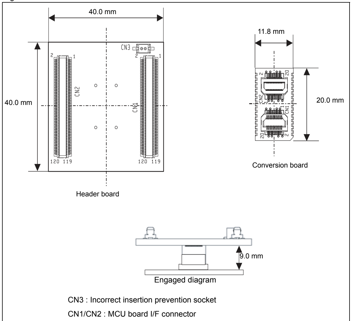
Figure 4-1. Header board and Conversion board dimensions
