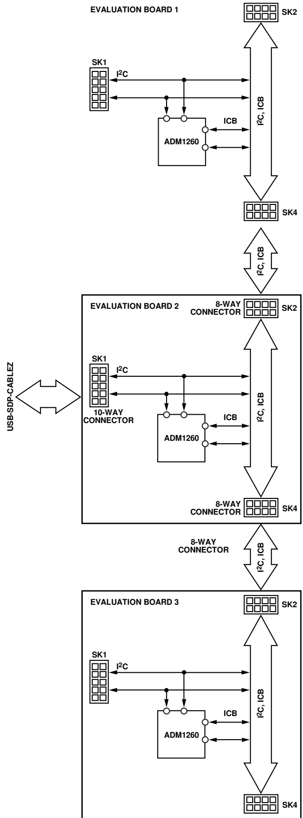
Figure 2. Multiple Boards Connection
