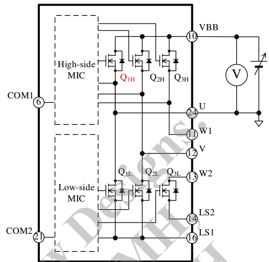
Figure 12-2. Typical Measurement Circuit for High-side Transistor ( Q_{IH} ) in U-phase
