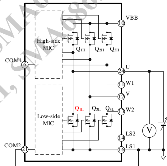
Figure 12-3. Typical Measurement Circuit for Low-side Transistor ( Q_{IL} ) in U-phase
