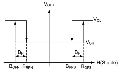
Figure 3. Switching characteristics
