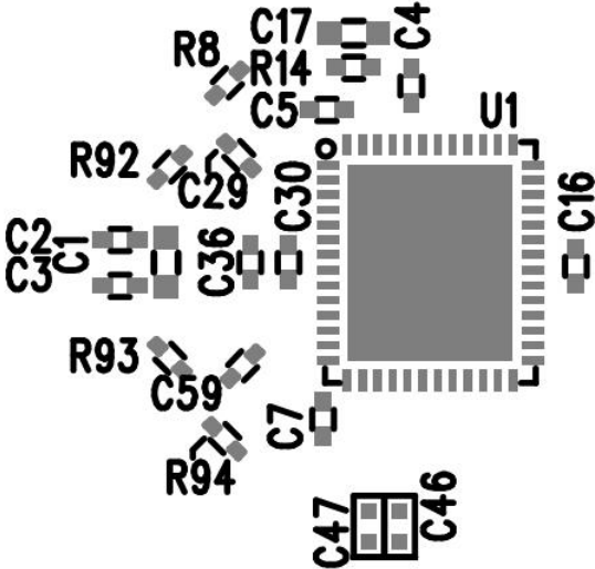
Silkscreen Top
