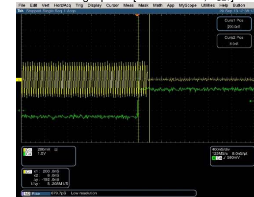
Attenuator Settling Speed [Min to Max, \tau_{SET} ]
