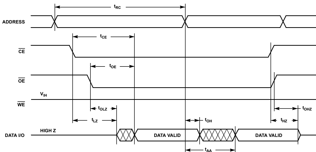
FIGURE 14. READ CYCLE
