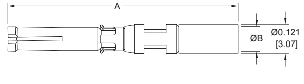
FEMALE CONTACT
