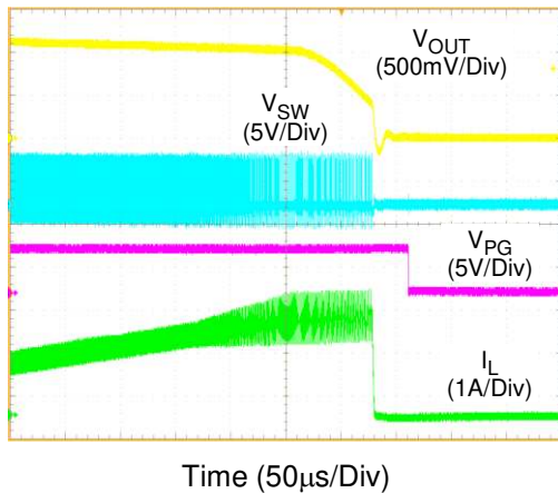
Figure 3. Over-Current Protection
