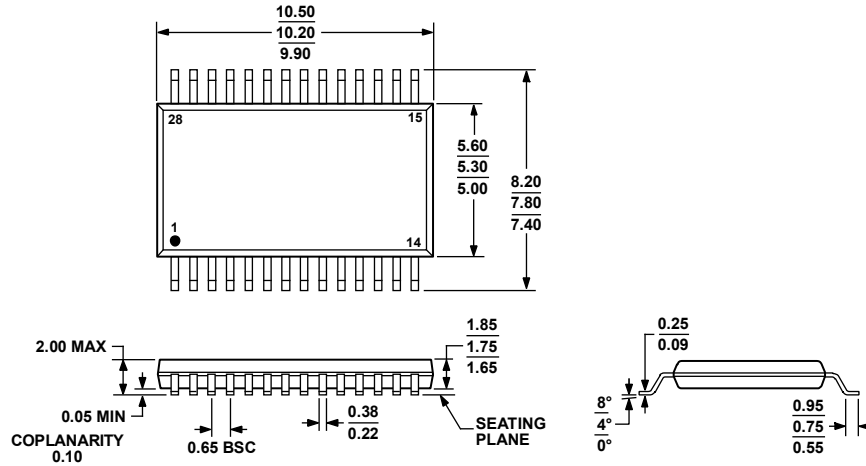
COMPLIANT TO JEDEC STANDARDS MO-150-AH Figure 31. 28-Lead Shrink Small Outline Package [SSOP] (RS-28) Dimensions shown in millimeters
