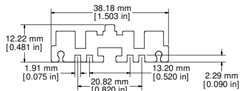
DETAIL BB
