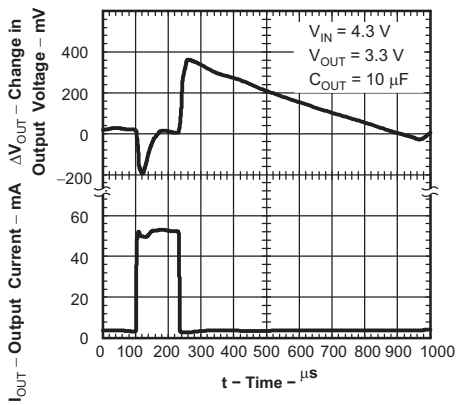
Figure 8-8. Load Transient Response for Legacy Chip
