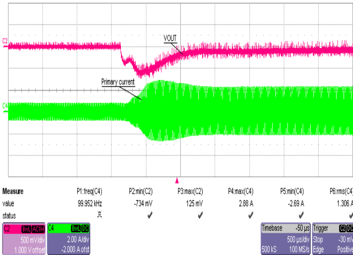
No Load to Full Load Step at 420Vdc
