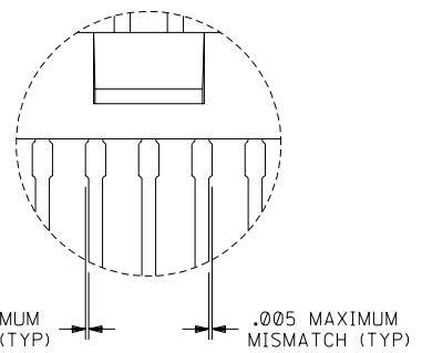
DETAIL "A" SCALE 10X
