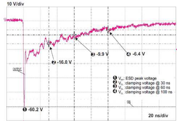
Figure 11. Typical ESD response to IEC 61000-4-2 -8kV contact
