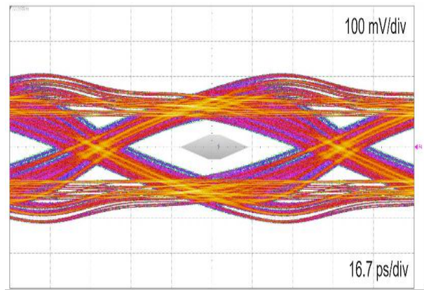
Figure 17. USB 3.2 Gen 2 - 10.0 Gbps eye diagram with ECMF02-2HSMX6 (with type C connector, reference cable, equalizer with ADC = 6 dB and DFE)
