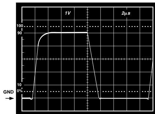
Figure 31. V_S = +5\text{ V} , 0\text{ V} ; Unity Gain Follower Response to 0 V to 5 V Step
