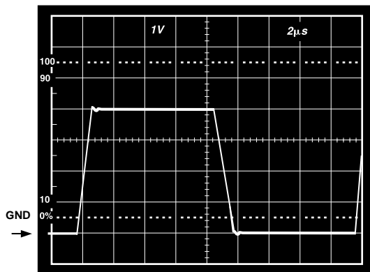
Figure 28. V_S = +5\text{ V} , 0\text{ V} ; Unity Gain Follower Response to 0 V to 4 V Step
