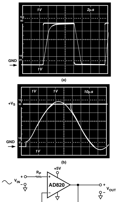
Figure 38. (a) Response with R_P = 0 ; V_{IN} from 0 to +V_S Figure 36. (b) V_{IN} = 0 to +V_S + 200 mV V_{OUT} = 0 to +V_S R_P = 49.9 k \Omega
