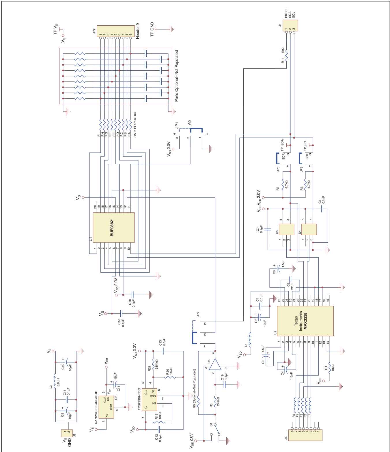
Figure 22. BUF08821EVM Schematic
