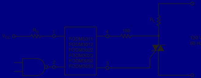
Figure 9. Resistive Load
