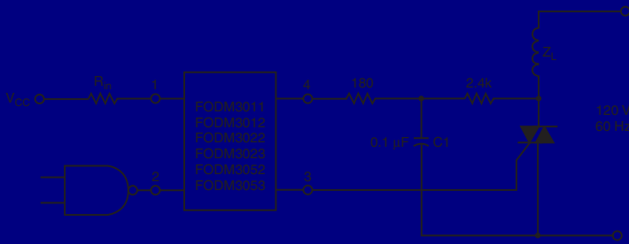
Figure 10. Inductive Load with Sensitive Gate Triac ( I_{LED} = 15mA )
