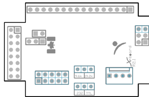
Figure 2: MOS X-Board
