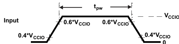
Figure 7-8. FlexRay Inputs
