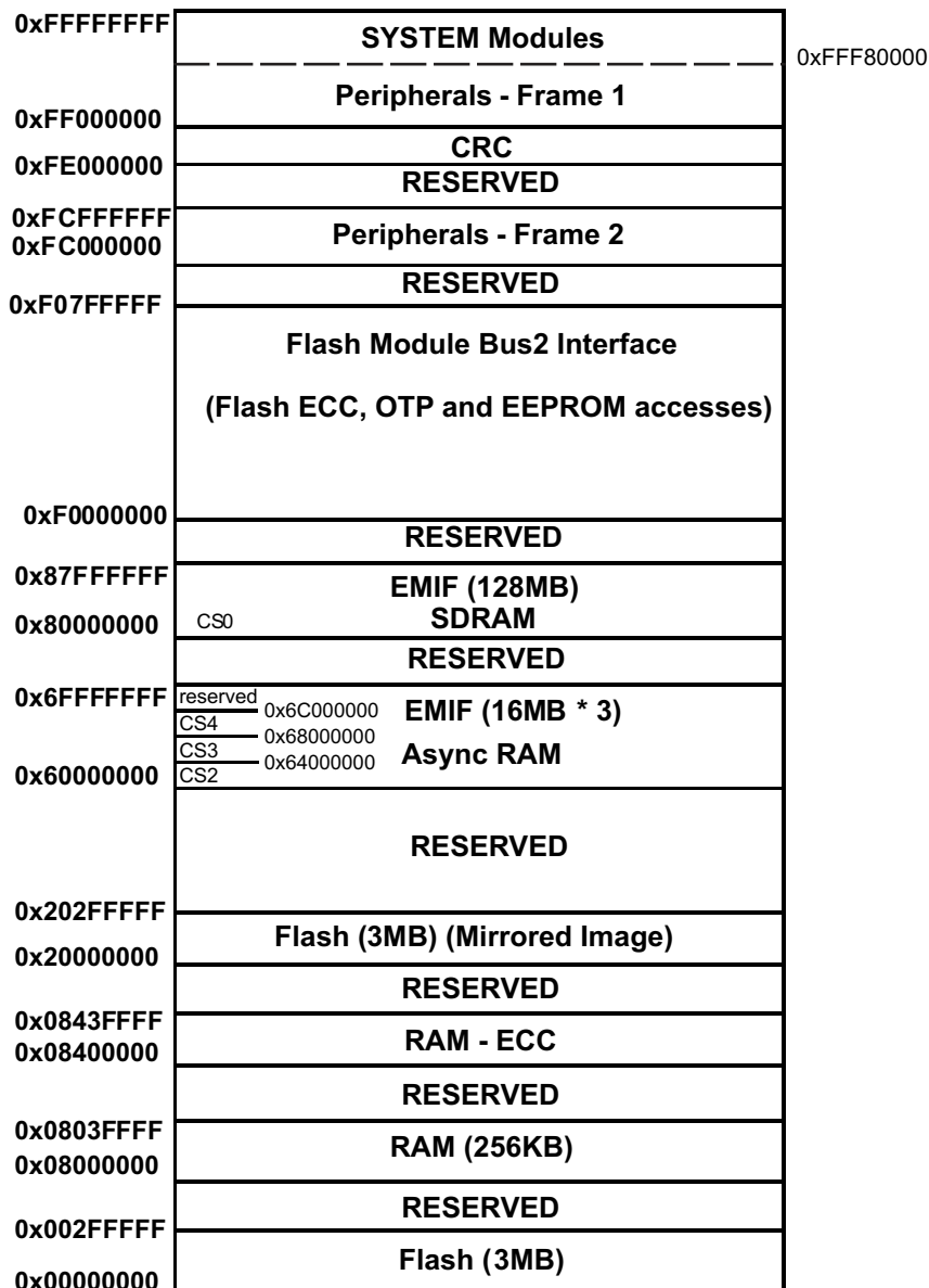
Figure 6-9. Memory Map
