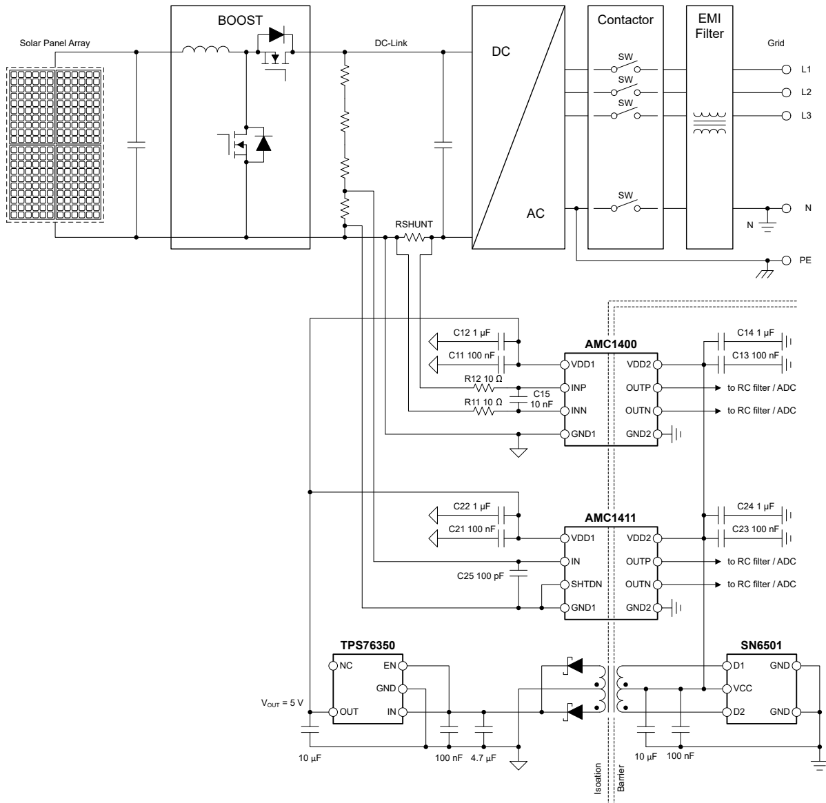
Figure 8-1. Using the AMC1400 for Current Sensing in a Typical Application
