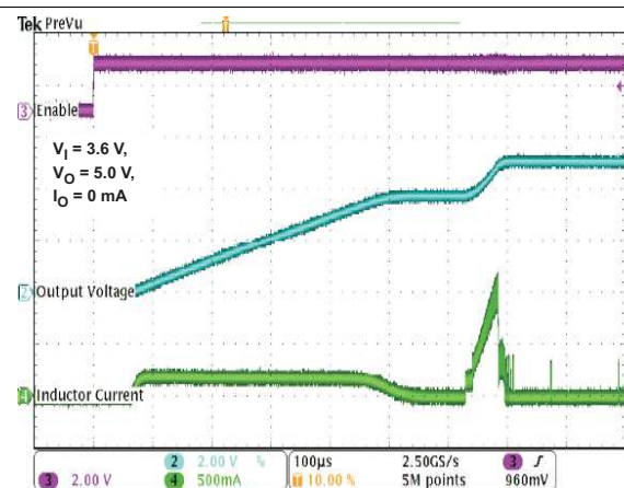
Figure 20. Start-Up
