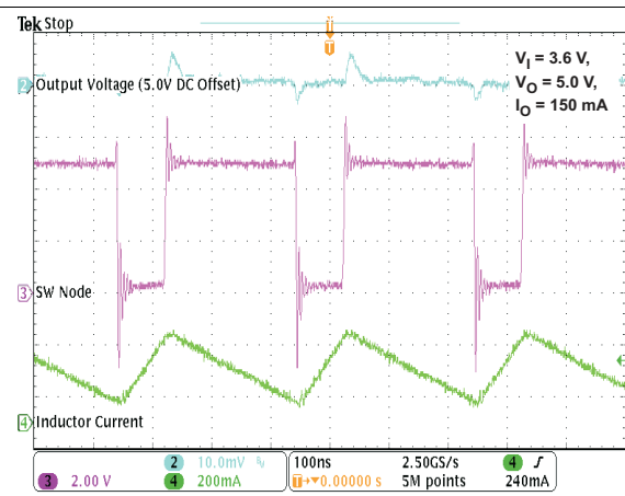
Figure 16. PWM Operation
