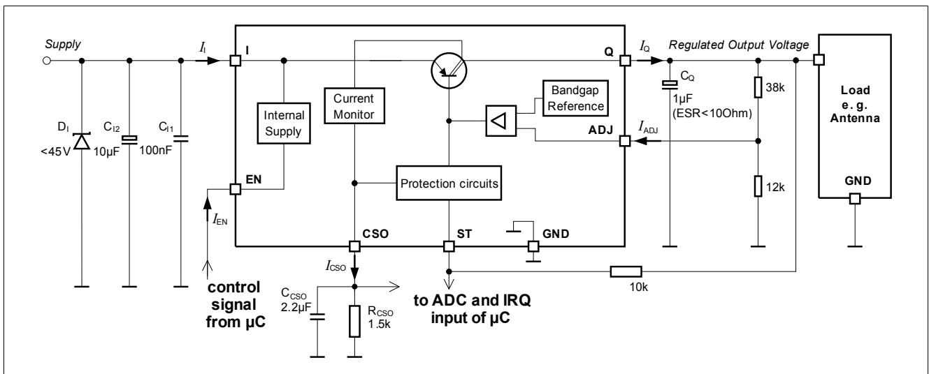
Figure 7 Application Diagram
