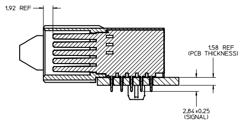
SECTION Z-Z
