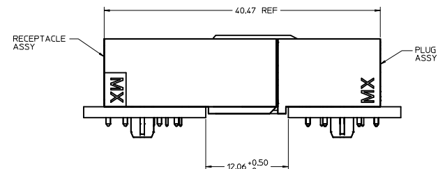
MATING PROFILE
