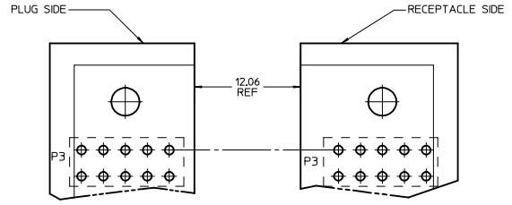
VIEW Z-Z (POWER CKTS ARE ALIGNED)
