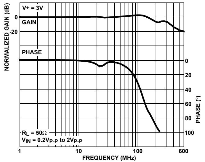
FIGURE 15. FREQUENCY RESPONSE
