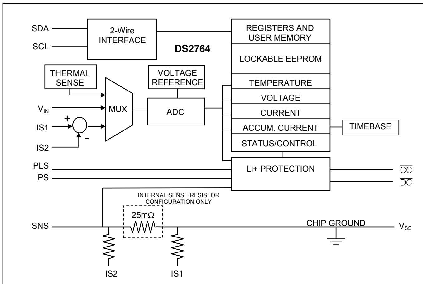
Figure 2. Block Diagram
