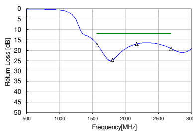
High-Port Return Loss
