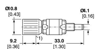
Part No. 2-1393670-2 ♦ Coupling Type A, B 2 , F 2
