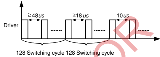
Figure 2— τ minoff at start-up Constant Voltage (CV) Operation
