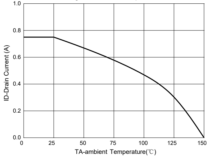
Fig. 10 - Current dissipation
