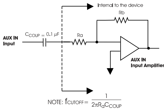
Figure 3: AUX IN Input Modes
