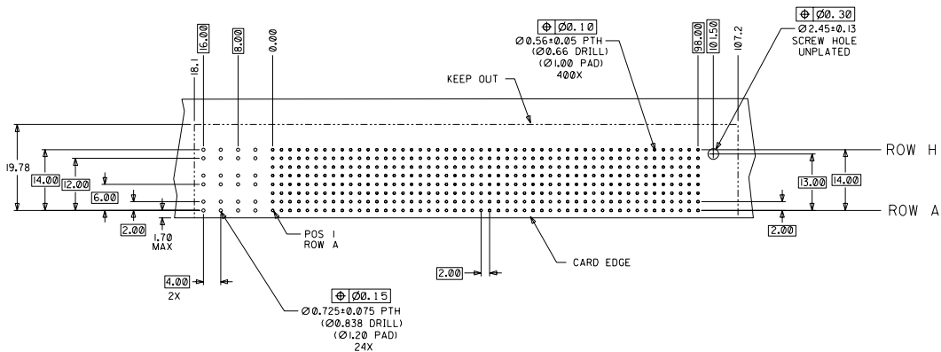
DAUGHTERCARD HOLE PATTERN (CONNECTOR SIDE)
