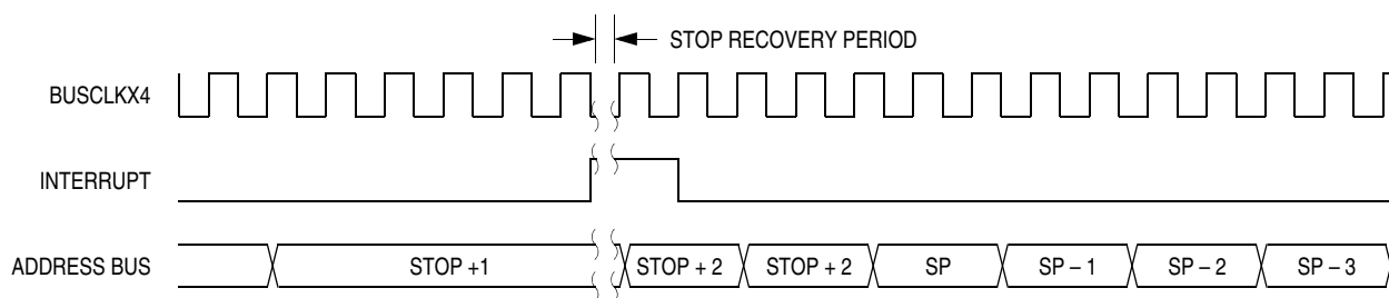
Figure 13-19. Stop Mode Recovery from Interrupt
