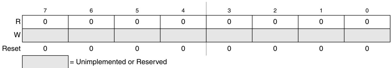
Figure 17-23. Flash Reserved6 Register (FRSV6)
