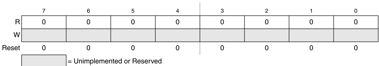
Figure 17-24. Flash Reserved7 Register (FRSV7)
