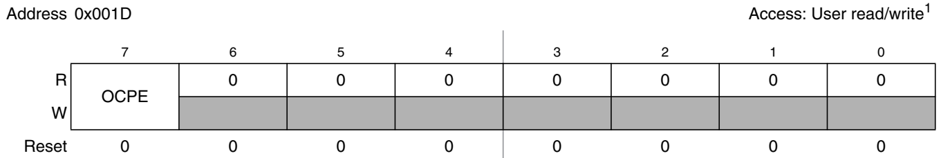
Figure 2-5. PIM Miscellaneous Register (PIMMISC)
