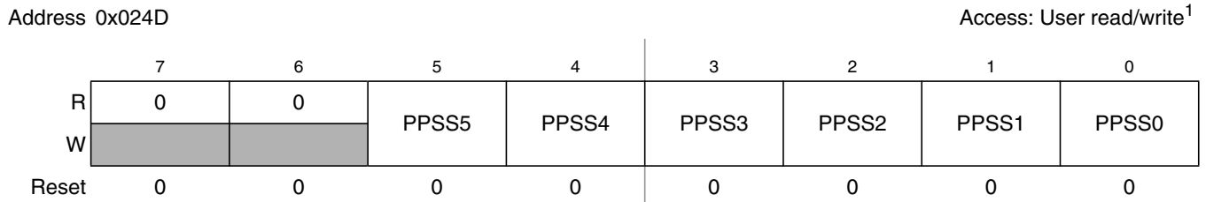
Figure 2-19. Port S Polarity Select Register (PPSS)
