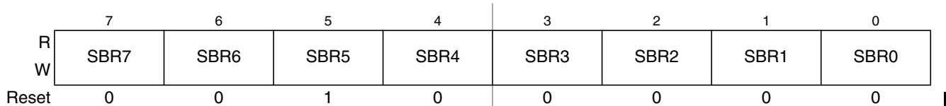
Figure 10-4. SCI Baud Rate Register (SCIBDL)
