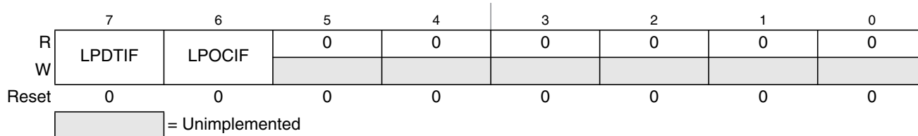
Figure 15-10. LIN Interrupt Flags Register (LPIF)
