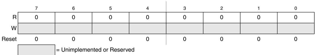
Figure 17-22. Flash Reserved5 Register (FRSV5)
