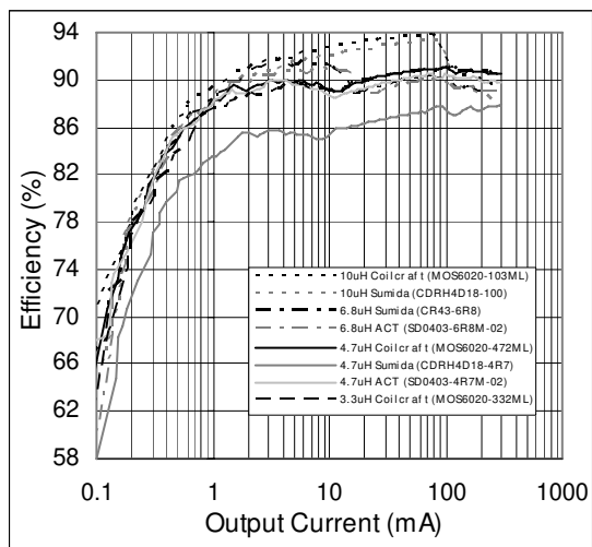
Figure 29. Efficiency Comparison of Different Inductors; V IN = 2.5V, V OUT = 3.3V
