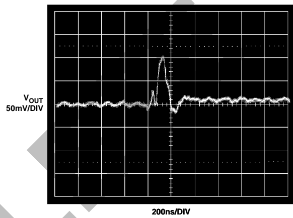
Figure 25. Glitch Impulse
