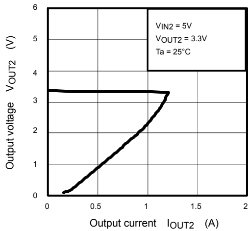
Overcurrent Protection (Series regulator section)
