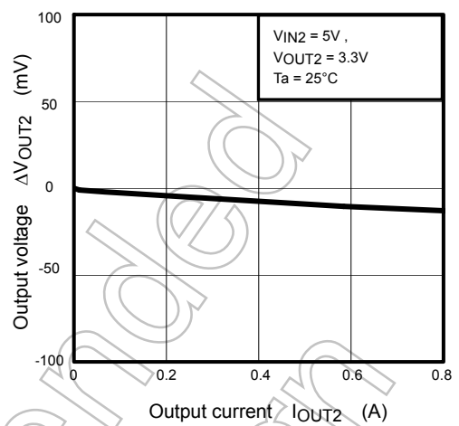
\Delta V_{OUT2} - I_{OUT2} (Series regulator section)
