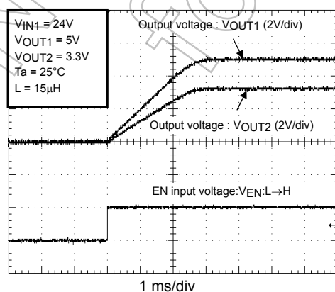
Startup Characteristics (Internal Soft-Start Time)
