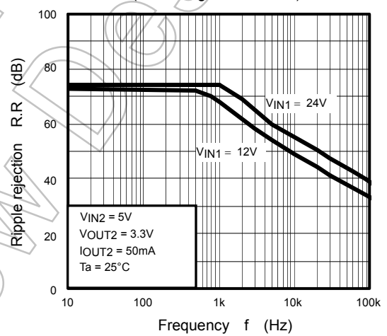
Ripple rejection (Series regulator section)
