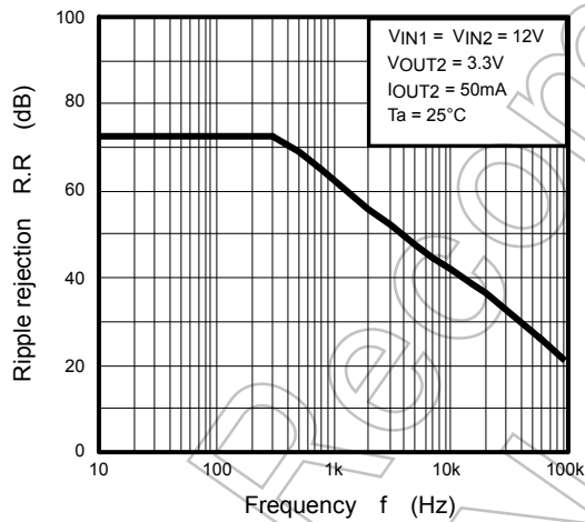
Ripple rejection (Series regulator section)
