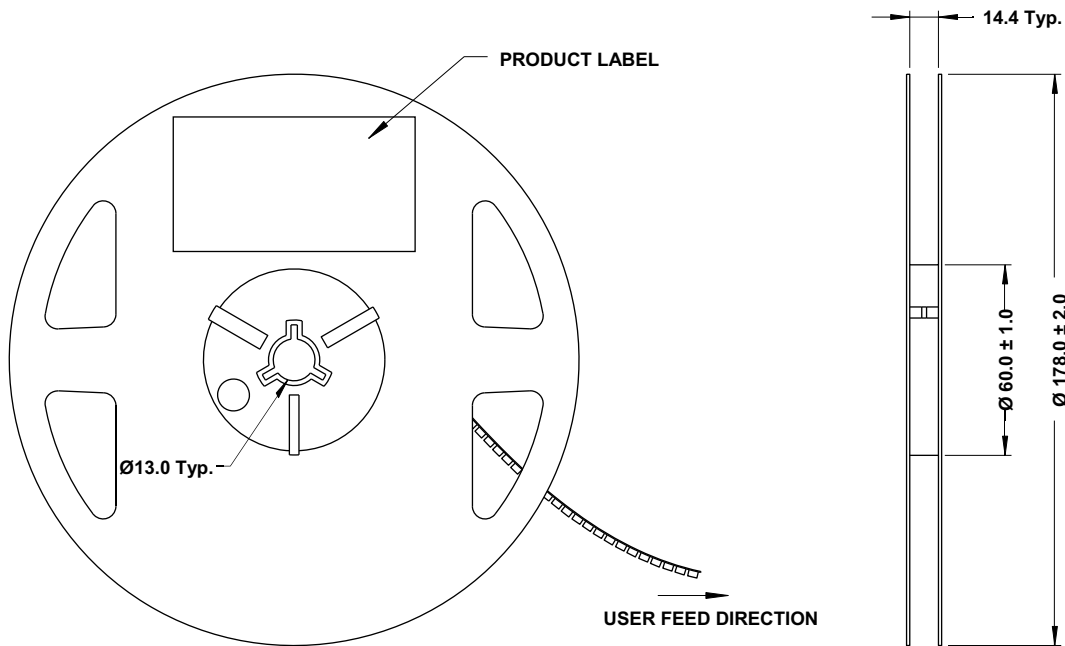
Figure 12: Reel Dimensions
