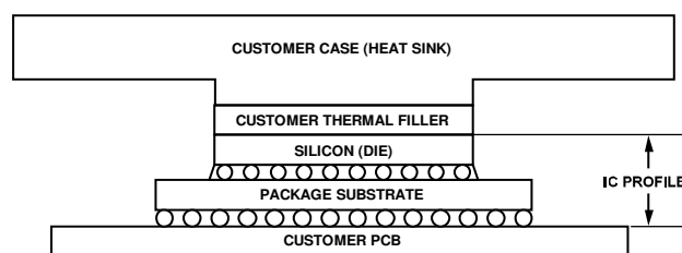
Figure 5. Typical Thermal Management Solution
