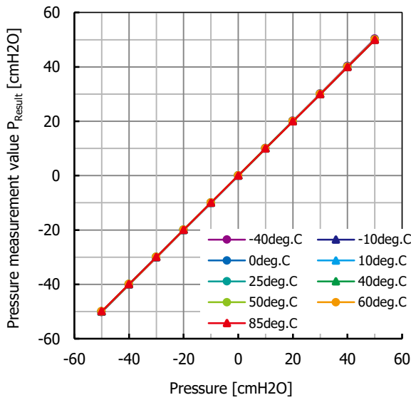
Fig.21.17 Pressure measurement value P_{\text{Result}} temperature characteristic
