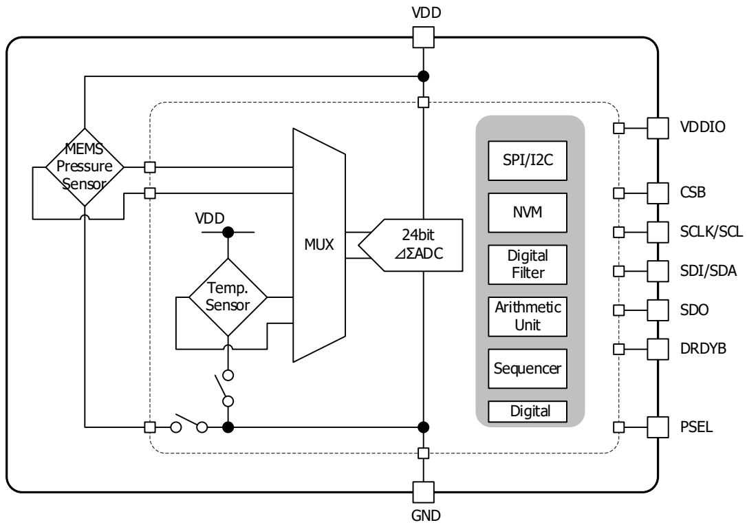
Fig.1 Block diagram
