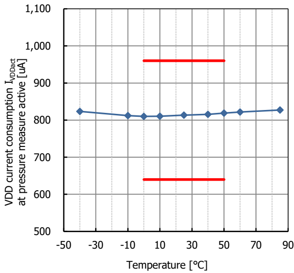
Fig.21.1 VDD current consumption I_{VDDact} at pressure measure active temperature characteristic
