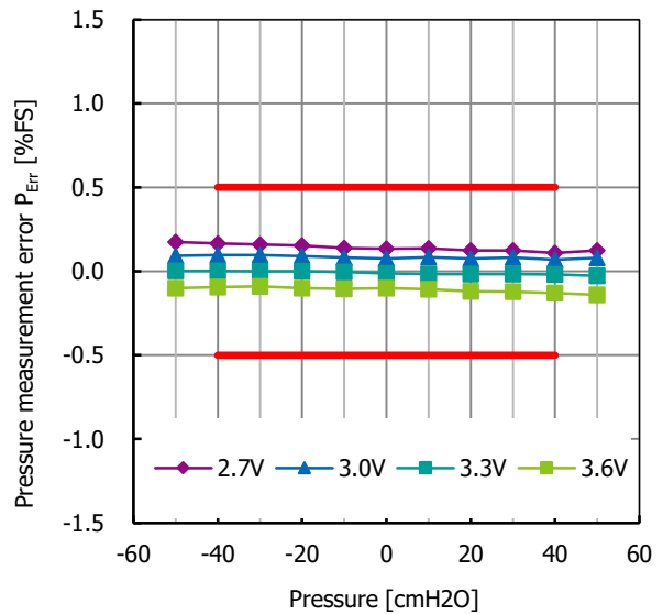
Fig.21.20 Pressure measurement error P_{\text{Err}} supply voltage characteristic
