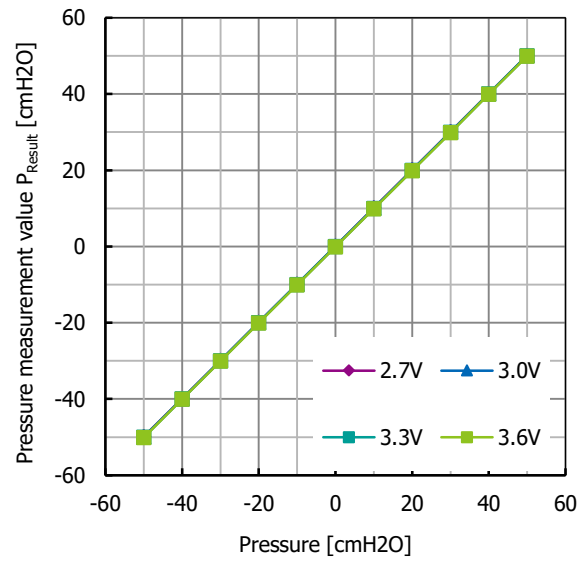
Fig.21.18 Pressure measurement value P_{\text{Result}} supply voltage characteristic
