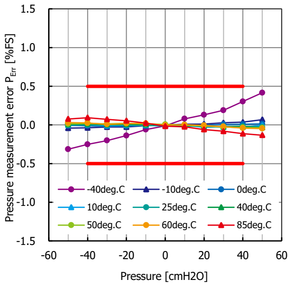
Fig.21.19 Pressure measurement error P_{\text{Err}} temperature characteristic
