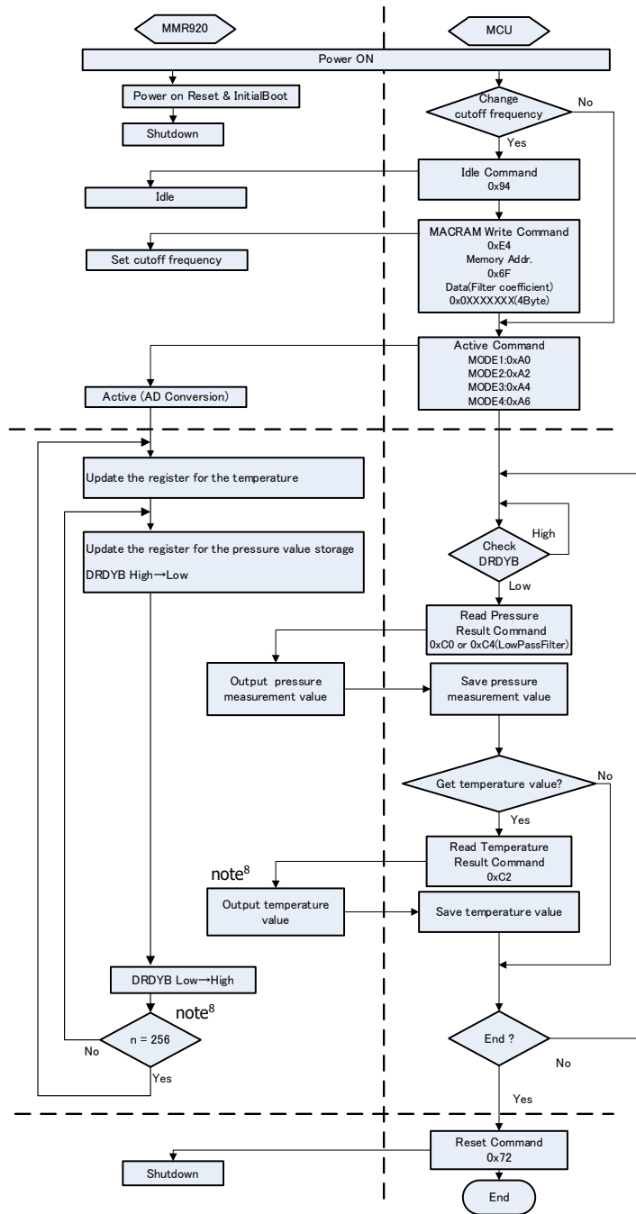
Fig. 6 Flow chart of pressure/temperature measurement
