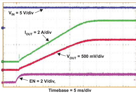
Figure 9-8. Start-Up With EN
