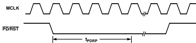
Figure 25. Power-Down/Reset Timing
